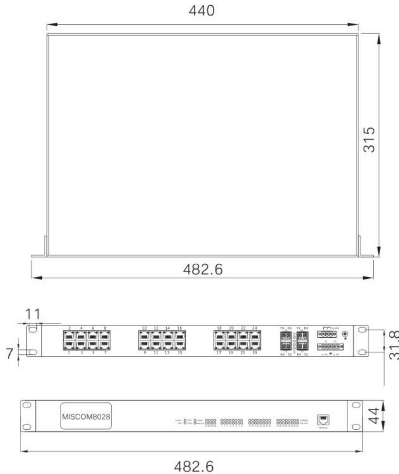
Rack mounting (Unit: mm)
